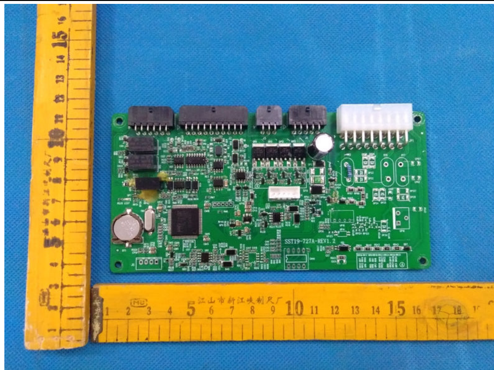
PCB general view-1 of BMS control board
