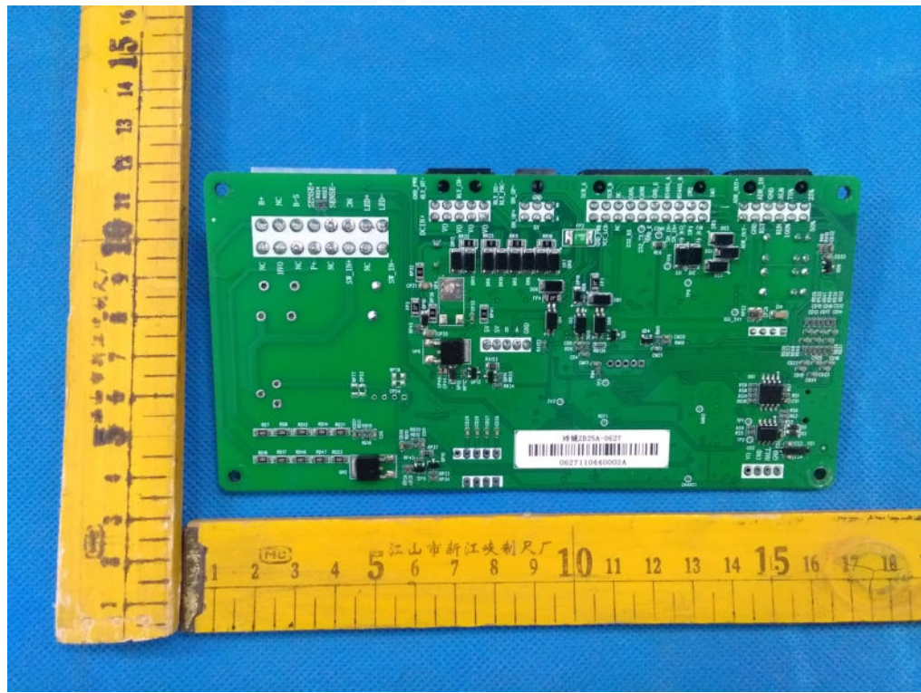
PCB general view-2 of BMS control board
