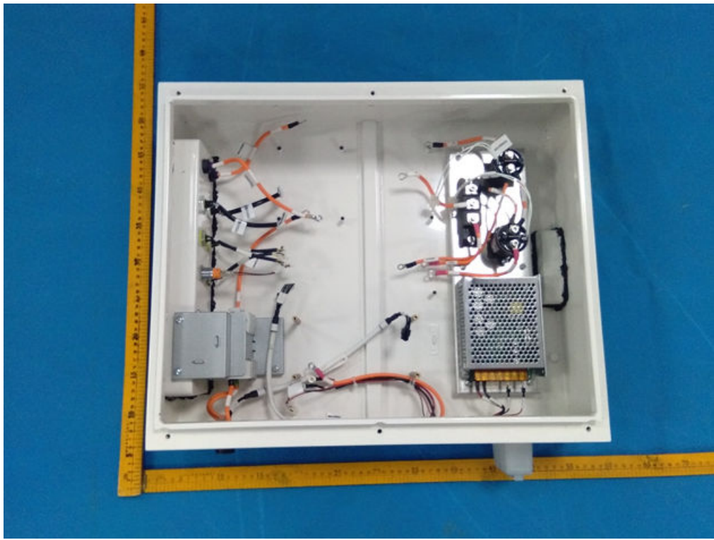
Internal view-2 of main control box
