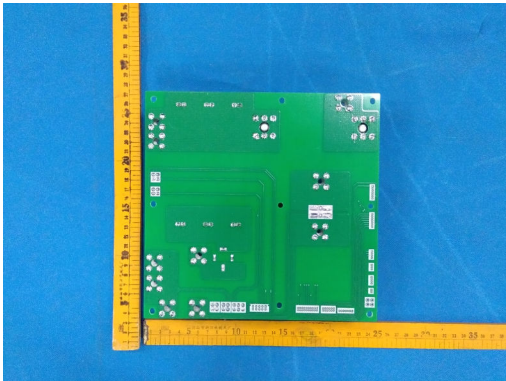
PCB general view-2 of main control box
