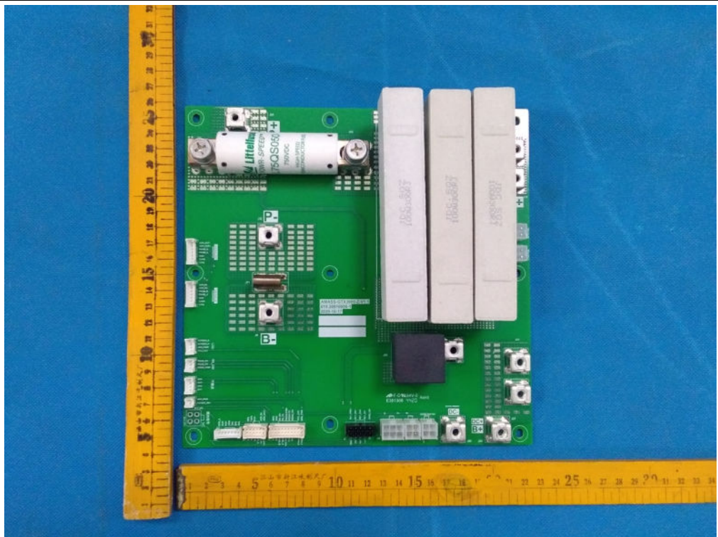
PCB general view-1 of main control box
