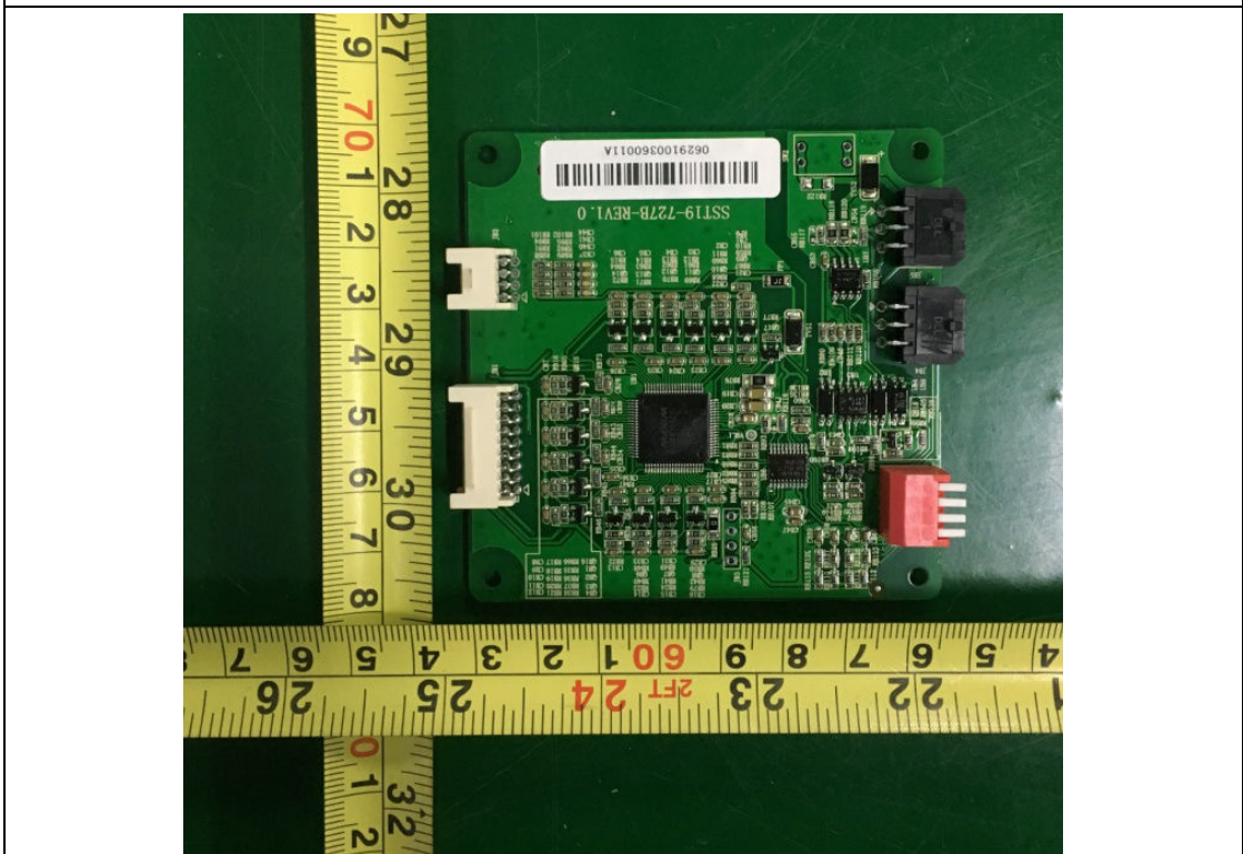
PCB general view-1 of battery module
