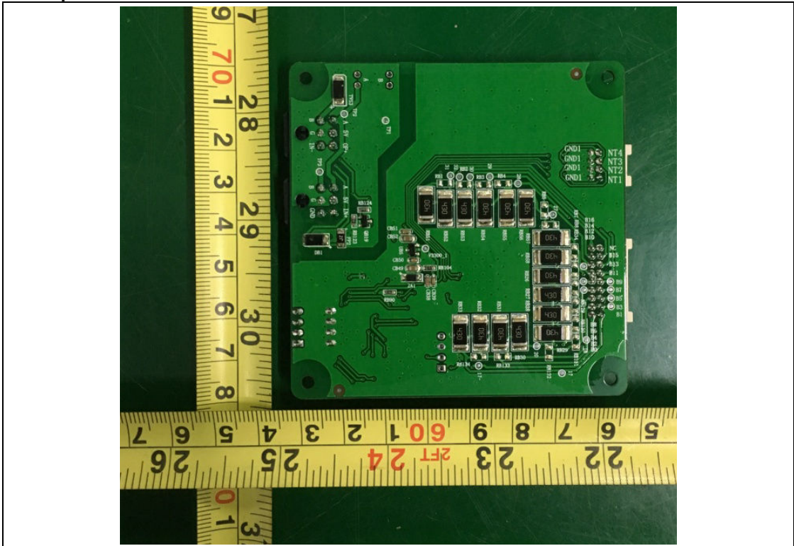
PCB general view-2 of battery module
